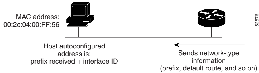
Figure 15 IPv6 Stateless Autoconfiguration
