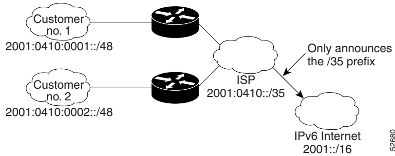
Figure 17 IPv6 Prefix Aggregation
