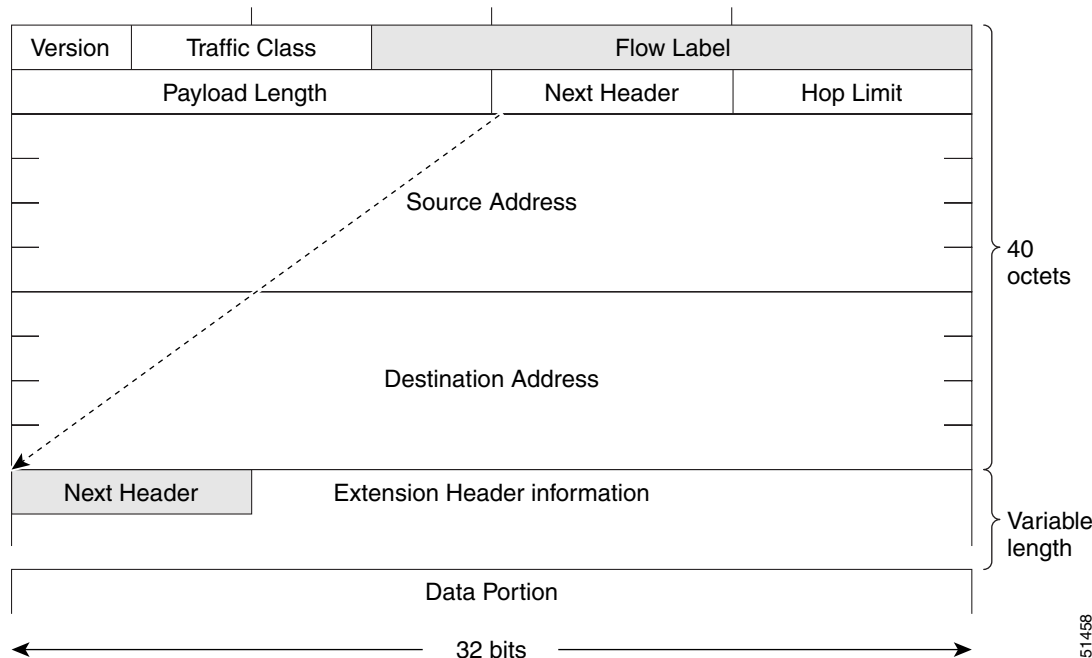
Figure 9 IPv6 Packet Header Format
