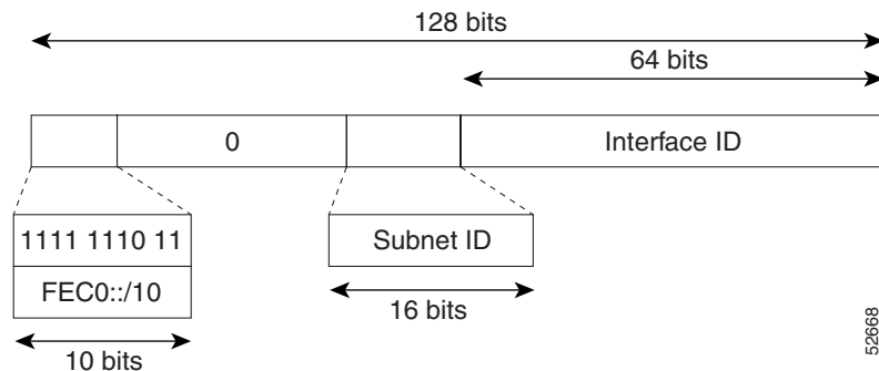
Figure 2 Site-Local Address Format
