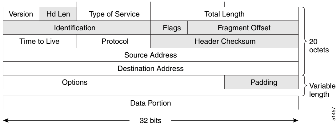
Figure 8 IPv4 Packet Header Format
