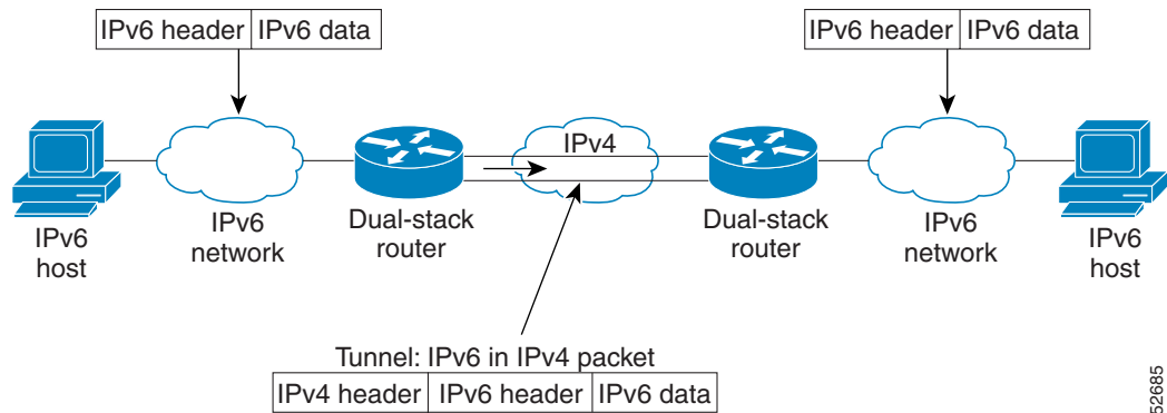
Figure 37 Overlay Tunnels
