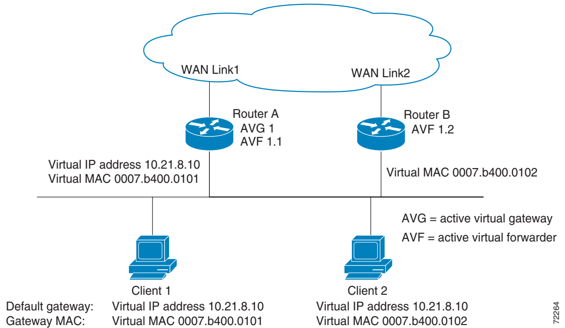
Figure 21 GLBP Topology
