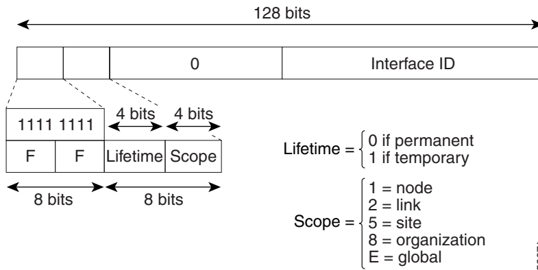
Figure 28 IPv6 Multicast Address Format
